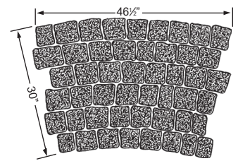
Tool D – 7½' to 10' radius
