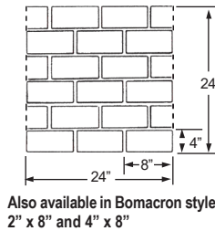
Running Bond Brick
