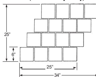
Running Bond Tile (Bomanite style only)
