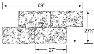
Running Bond Coquina
