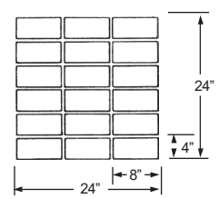
Stacked Bond Brick
