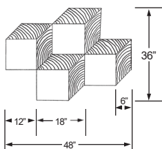
3-D Graphics
