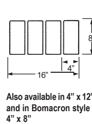
Soldier Course Brick
